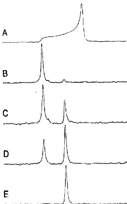
Fig. 1. ^{31}\text{P} -NMR spectrum of POPE multilamellar dispersions acquired at 30^\circ\text{C} (A). Representative ^{31}\text{P} -NMR spectra of DOPE macroscopically oriented at an angle of 0^\circ (angle between bilayer normal relative to external magnetic field) at 0^\circ\text{C} (B), 8^\circ\text{C} (C), 13^\circ\text{C} (D) and 23^\circ\text{C} (E). Number of acquisitions = 1024 (A), 64 (B-E). The plot width is 10 kHz.
