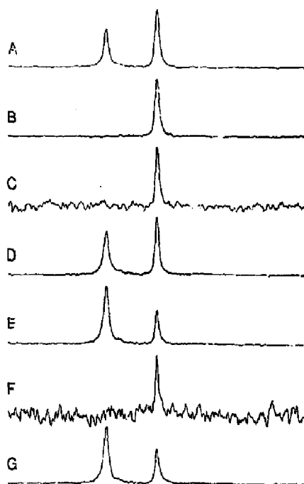
Fig. 3. Hahn echo (A, D, E, G) and 1D exchange spectra (B, C, F) of oriented DOPE (0°-orientation) at 15°C (A–D) and 18°C (E–G) for t_{\text{mix}} = 500 ms (B), 3 s (C) and 4 s (F). (A) and (D) were acquired immediately prior to and following the acquisition of (B) and (C), respectively and (E) and (G) were acquired immediately prior to and following the acquisition of (F). Number of acquisitions = 32 (A, D, E, G), 64 (B), 256 (C), 1024 (F). The plot width is 10 kHz.
