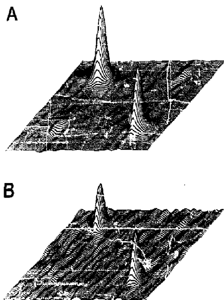
Fig. 2. 2D exchange spectra of oriented DOPE (0°-orientation) at 9°C and 14°C for t_{\text{mix}} = 500 ms and 2 s, respectively (A, B). The plot width is 3.2 kHz in both dimensions.
