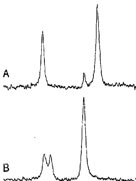
Fig. 5. Representative ^{31}\text{P} -NMR spectra of DOPC/MO (1:1) (A) and DOPC/DOPE/cholesterol (1:1:2) (B) at 43°C (0° orientation). The cubic I_2 phase of (A) is distinguished from the L_\alpha and (transient) H_{II} phases, as seen by comparison with the L_\alpha/H_{II} phases in (B). The plot width is 6 kHz.
