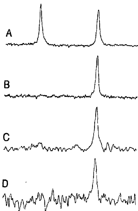
Fig. 6. Lahn echo (A) and 1D exchange spectra (B–D) of DOPC/MO (3:7) ( l_0 -orientation) at 3°C for t_{\text{mix}} = 100 ms (B), 2 s (C) and 4 s (D). Number of acquisitions = 128 (A, B), 256 (C), 1200 (D). The plot width is 6 kHz.
