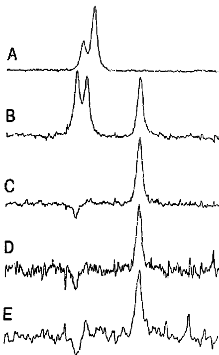
Fig. 4. (A) Representative ^{31}\text{P} -NMR spectrum of DOPE/DOPC (7:3) in the L_\alpha phase at 33°C (0° orientation). (B) Representative ^{31}\text{P} -NMR spectrum of DOPC/DOPE/cholesterol (1:1:2) at 33°C (0° orientation). (C–E) 1D exchange spectra of DOPC/DOPE/cholesterol (1:1:2) at 33°C (0° orientation) for t_{\text{mix}} = 100 ms (C), 2 s (D), 3 s (E). Number of acquisitions = 96 (A), 128 (B, C), 800 (D), 1648 (E). The plot width is 6 kHz. The slight inversion of the DOPC resonance is a result of setting the experiment to nullify the DOPE resonance at short mixing times.
